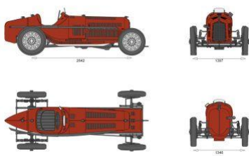
Alfa Romeo P3 (1933)
