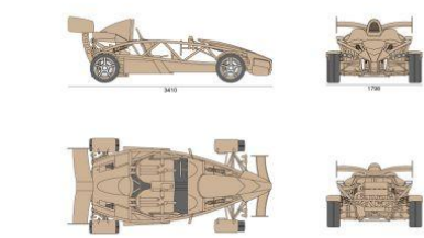
Ariel Atom
