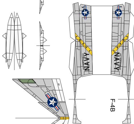
MDD F4B Phantom II
