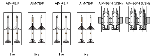
F-4N/J/S Phantom II (grey undersides)
